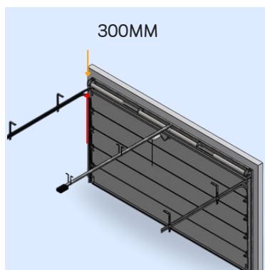
Standard Lift
