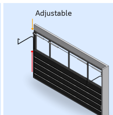
High Lift
