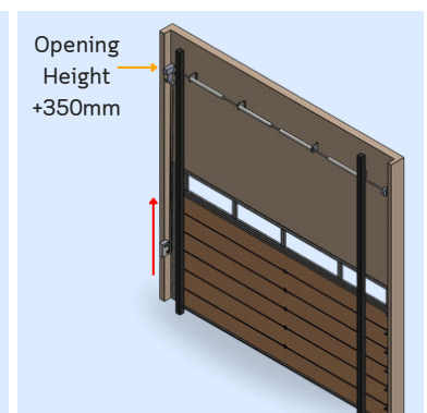
Vertical Lift
